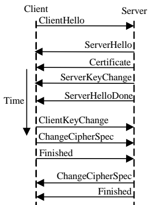
Fig.3 Procedure of TLS handshake
