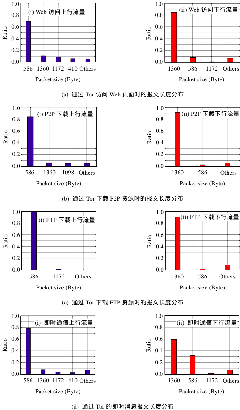
Fig.12 Packet size distribution of Tor traffic
