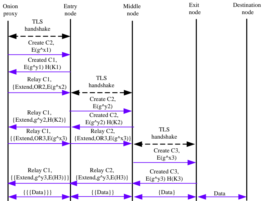
Fig.2 Procedure of circuit creation on Tor
