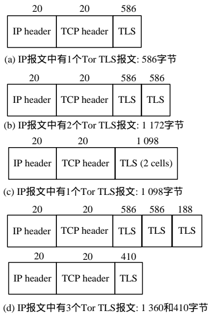
Fig.8 Packet format of typical size
